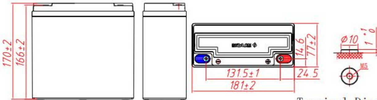
Terminal Dimensions
